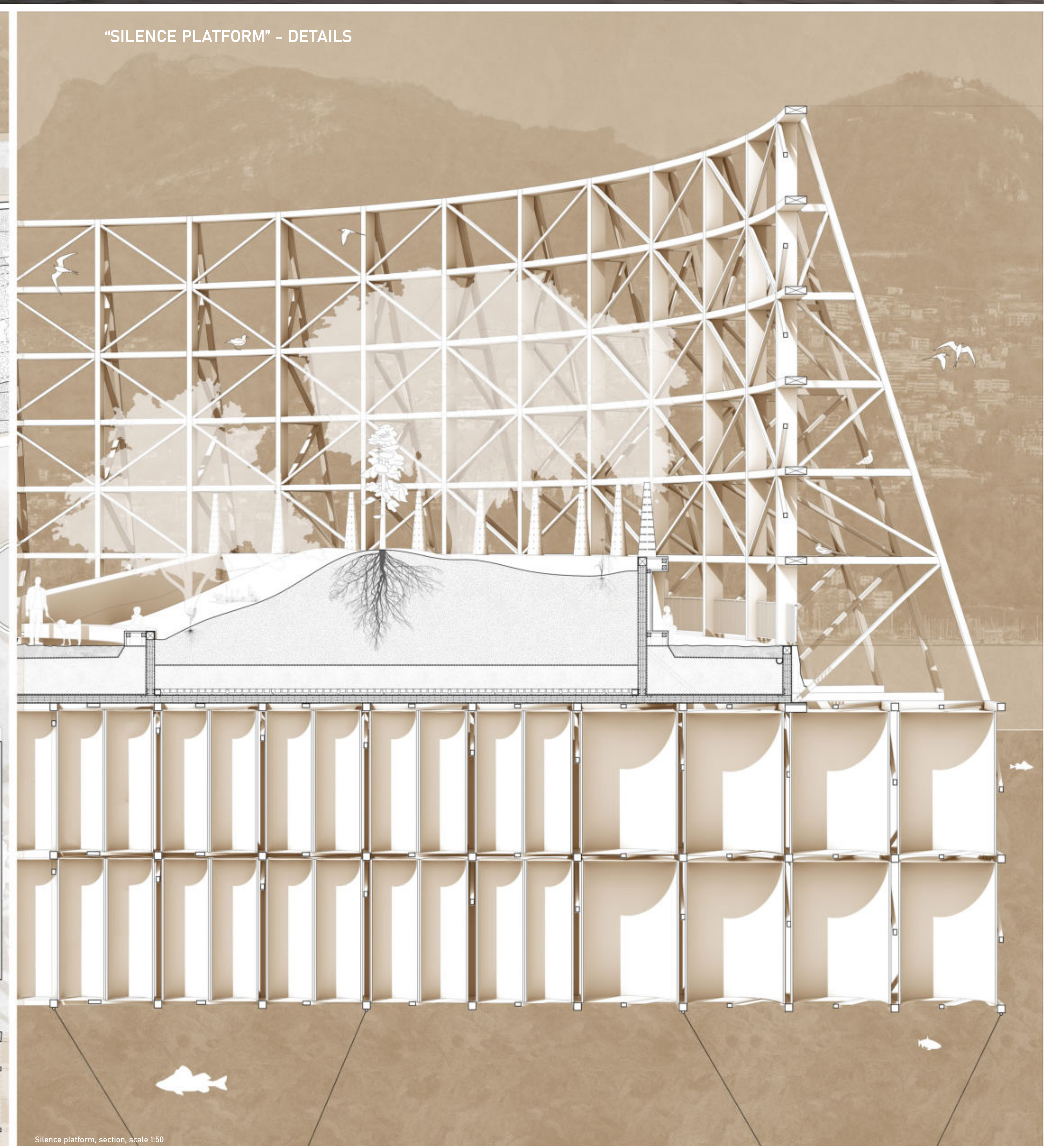
Silence platform, section, scale 1:50
